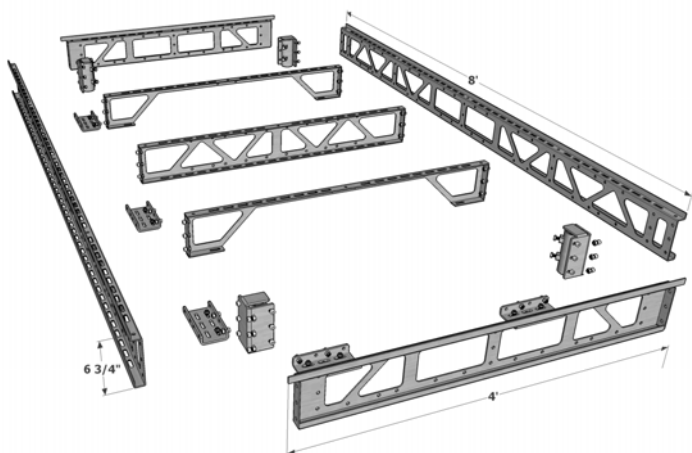
4' x 8' Tdeck+™ explosion with Corner Bracket Pipe Sockets and five Marriage Brackets
