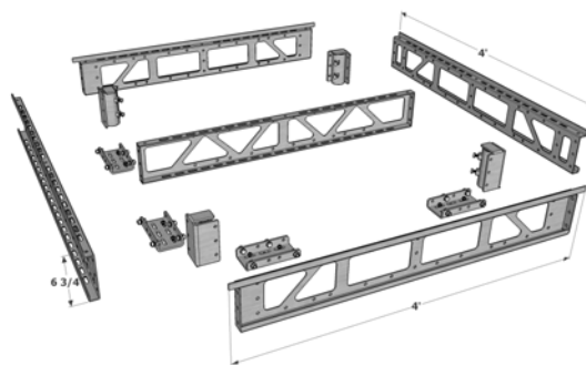
4' x 4' Tdeck+™ explosion with Corner Bracket Pipe Sockets and four Marriage Brackets
